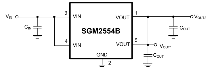
C IN = 1µF, C OUT = 470µF (Low ESR) on M/B C IN = 1µF, C OUT = 330µF (Low ESR) on Notebook C IN = 10µF, C OUT = 1µF on USB Device
