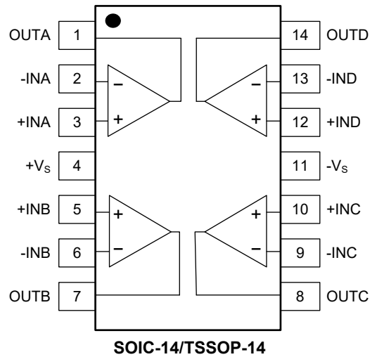
SGM8538 (TOP VIEW)
