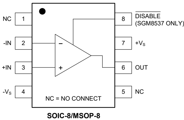
SGM8535/7 (TOP VIEW)
