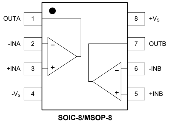
SGM8536 (TOP VIEW)
