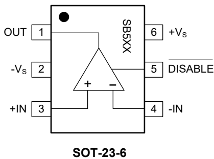
SGM8537 (TOP VIEW)
