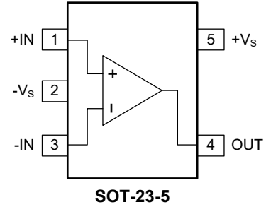
SGM8535BYN5G/TR (TOP VIEW)
