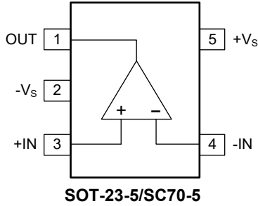
SGM8535AYN5G/TR (TOP VIEW) SGM8535YC5G/TR (TOP VIEW)
