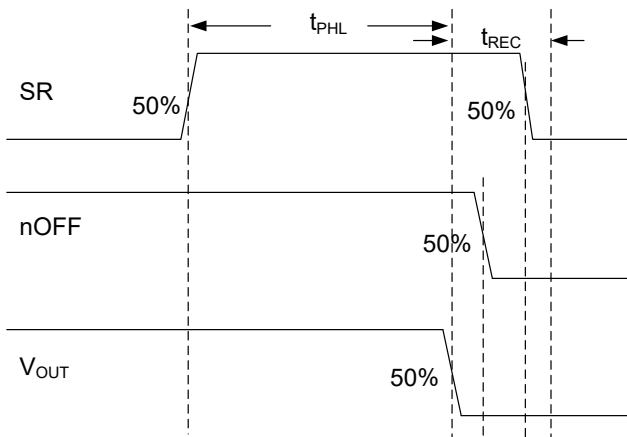
图 11. Timing Diagram (SR + nOFF vs. V OUT ) 1
