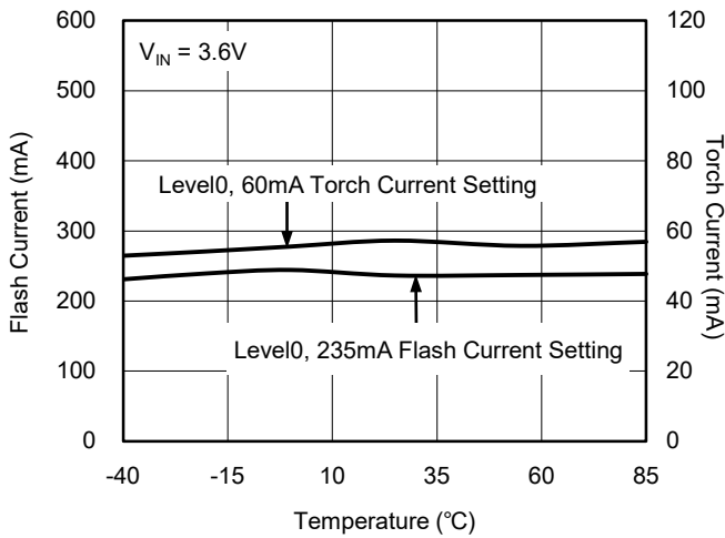
Flash Current and Torch Current vs. Temperature
