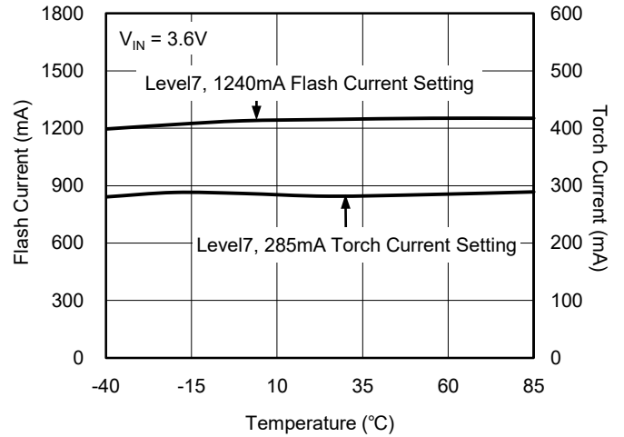
Flash Current and Torch Current vs. Temperature (37891A)
