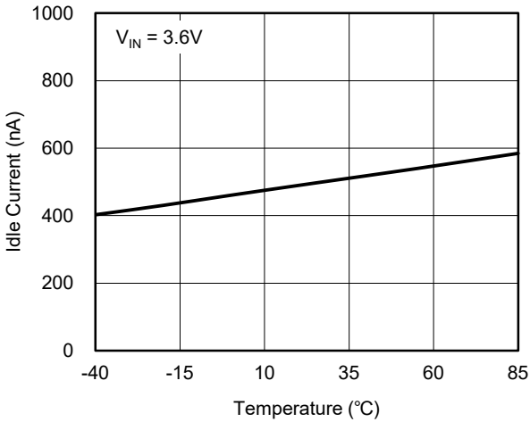
Idle Current vs. Temperature
