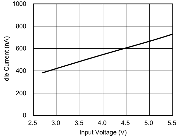
Idle Current vs. Input Voltage
