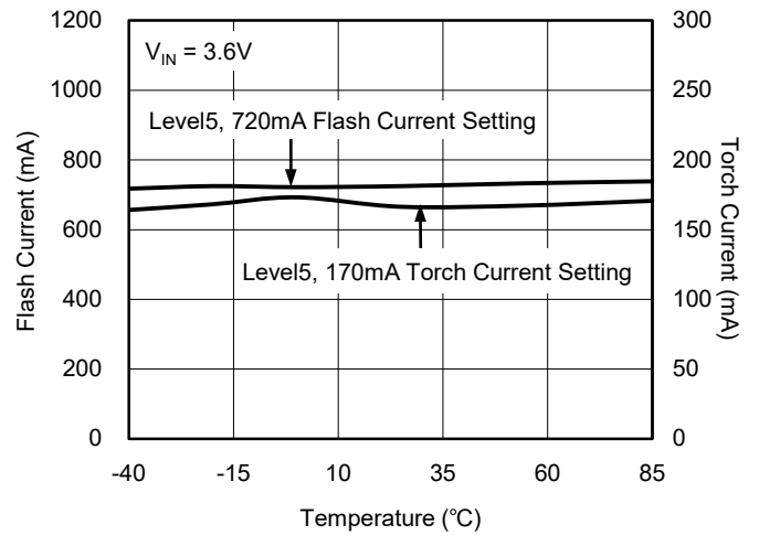
Flash Current and Torch Current vs. Temperature
